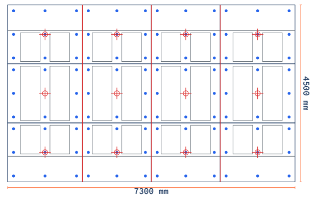
RT-B-Z 7.3 × 4.5 7300 × 4500 mm
